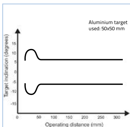
Maximum target inclination (models with discrete output)
